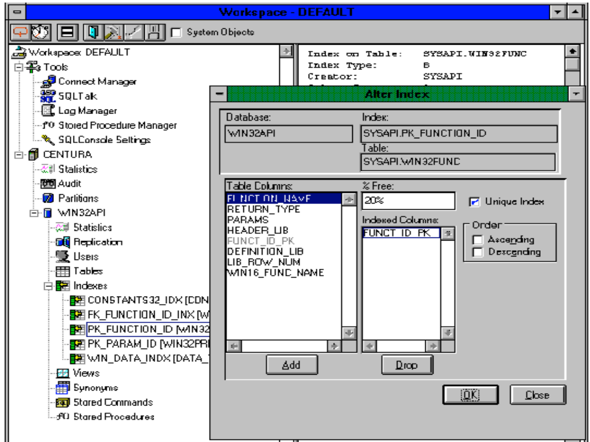
Figure 2: Alter index screen from SqlConsole 6.1. Notice the included columns and the Unique Index check box.
