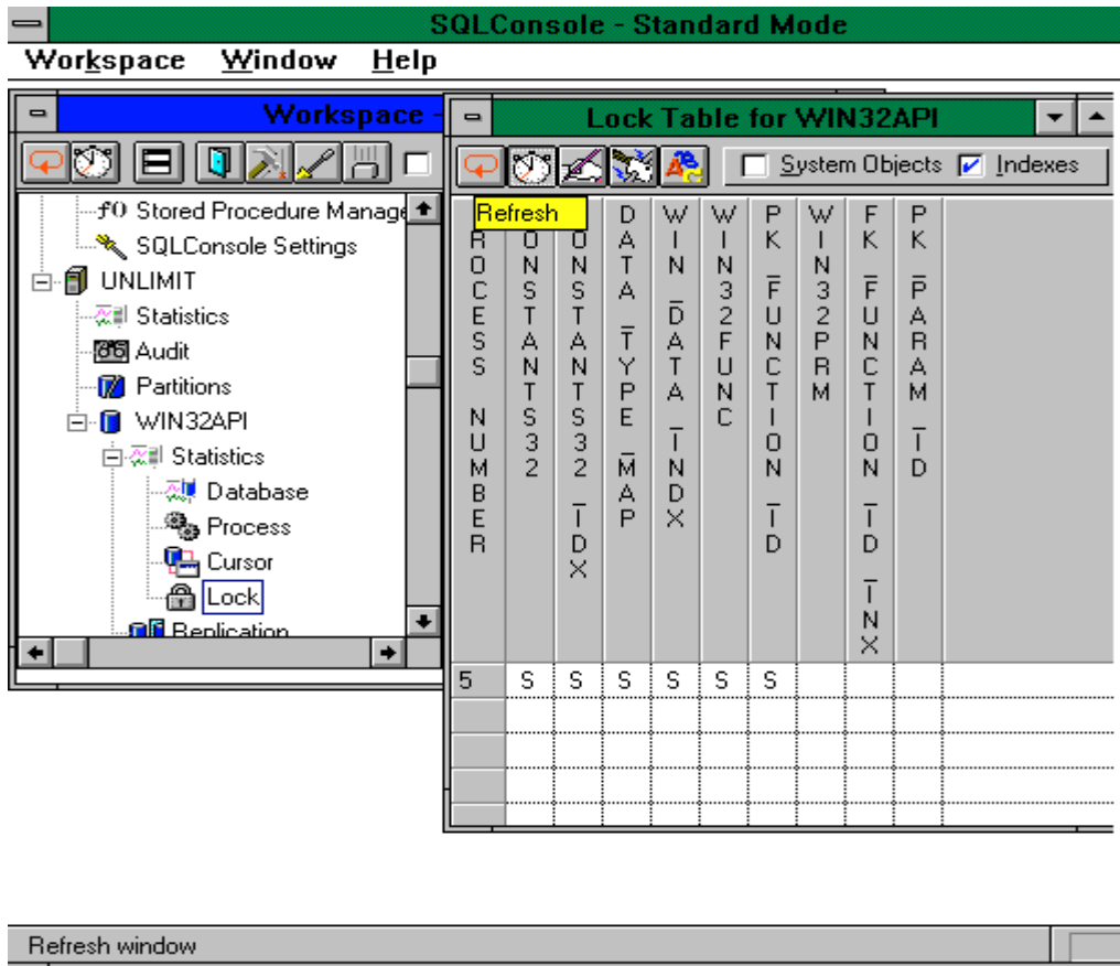
Figure 1. Lock screen from SqlConsole 6.1 showing the indexes and tables during a check database. Notice the shared ( S ) locks being held as the tables are being checked. At the time of the picture, PK_FUNCTION_ID was being checked. Indexes are noted by the X at the end of the name.
