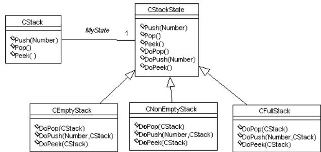
Figure 1. The State pattern.
