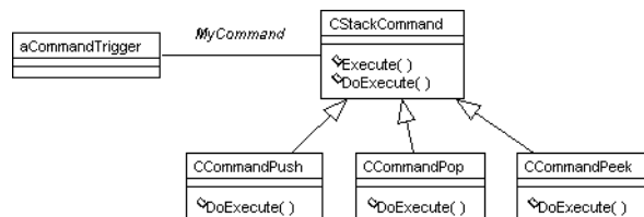
Figure 3. The Command pattern.
