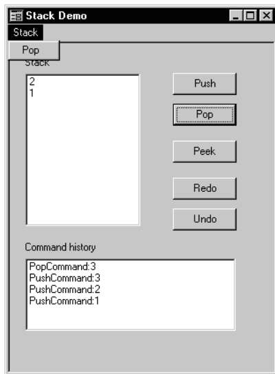
Figure 2. The user interface.
